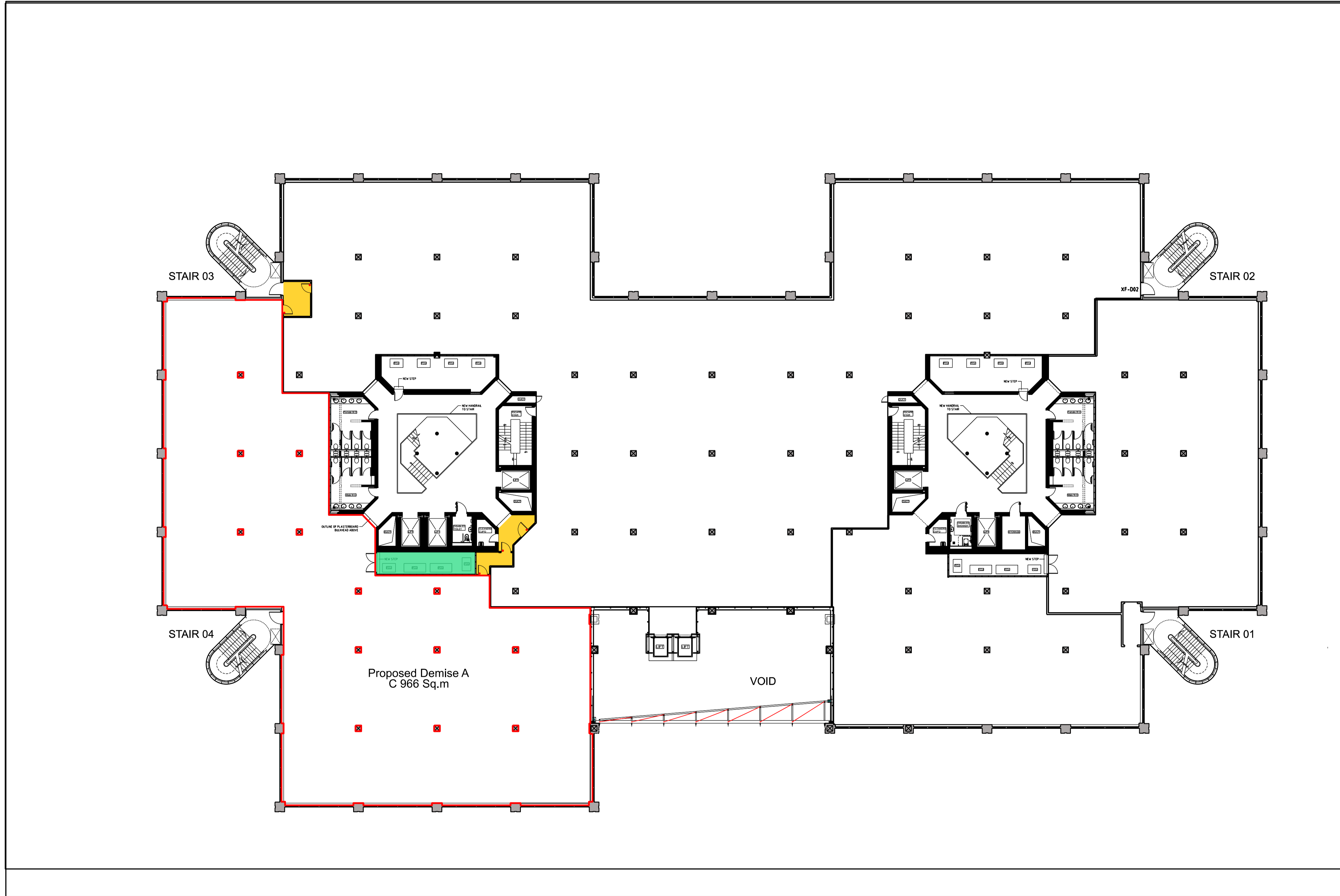
02 Proposed First Floor Plan - Demise 3 1:200 @ A1
