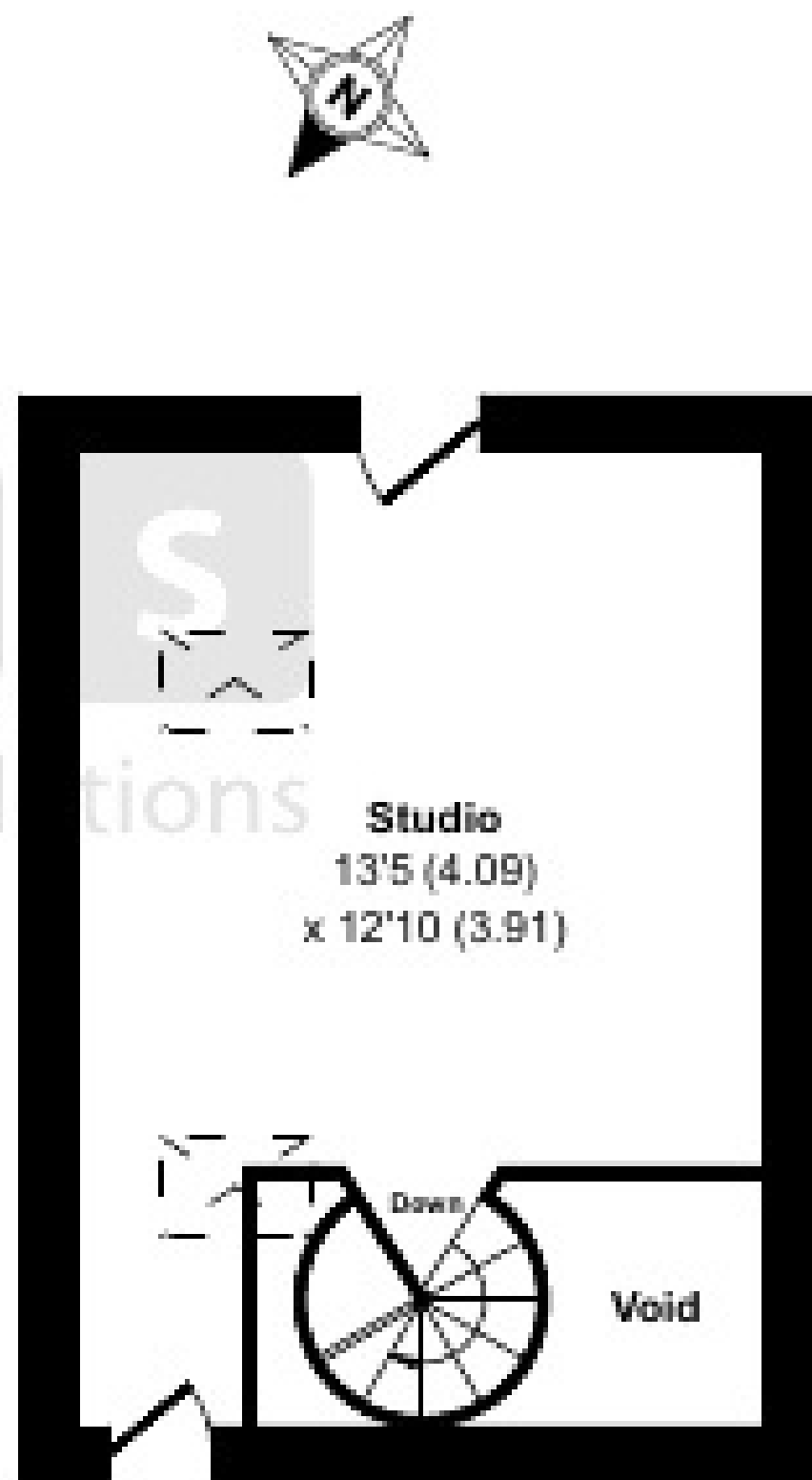
FIRST FLOOR
