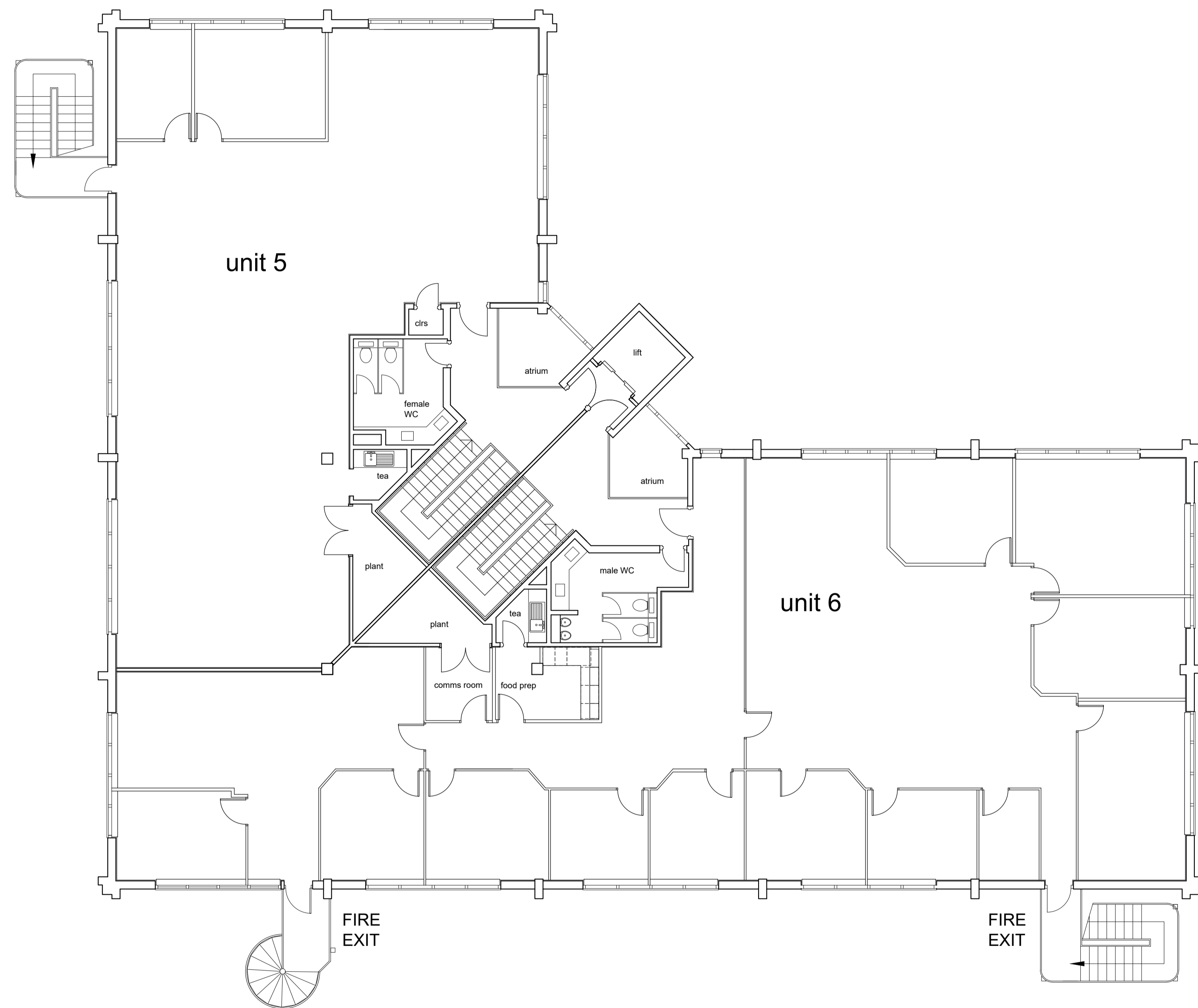
first floor plan as existing
