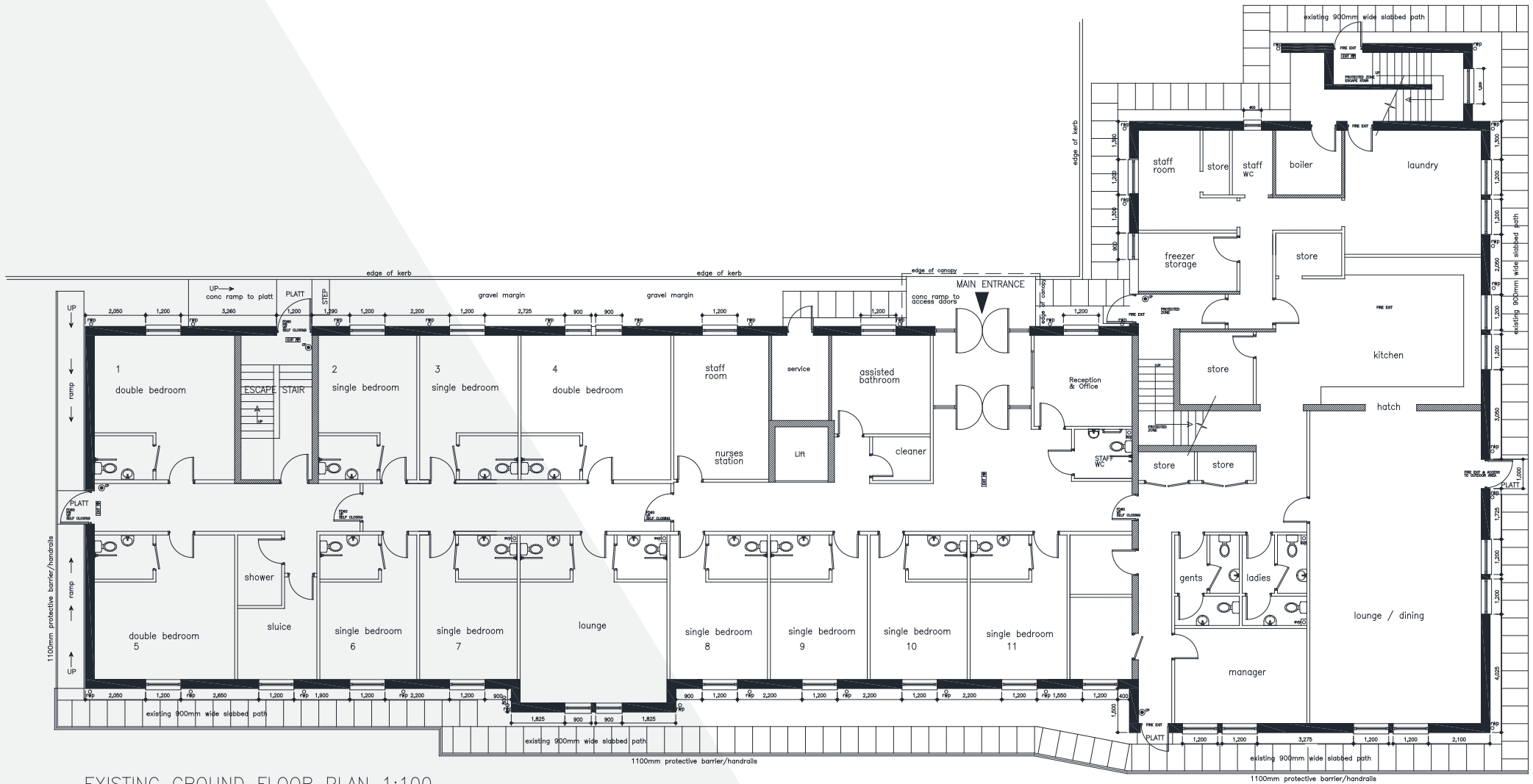
EXISTING GROUND FLOOR PLAN 1:100 Existing Accommodation on Ground floor – 11no. residential rooms
