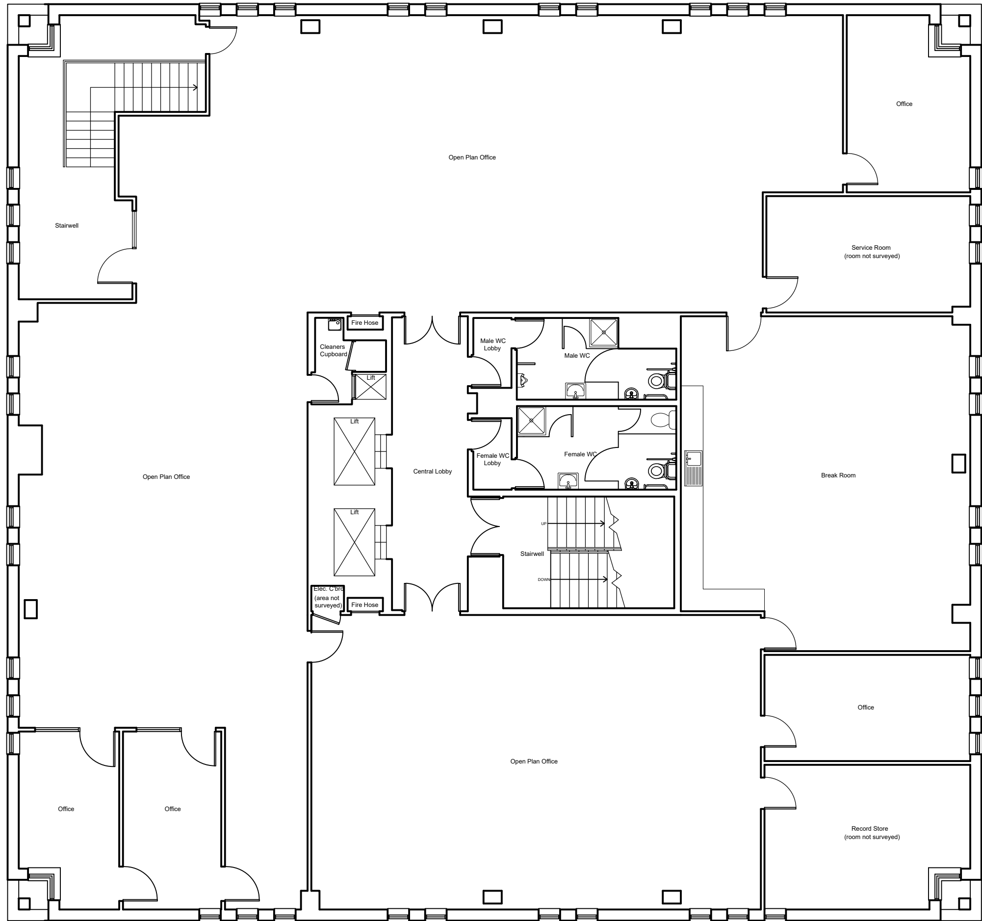
FIRST FLOOR PLAN - AS EXISTING SCALE: 1:100 @ A3
