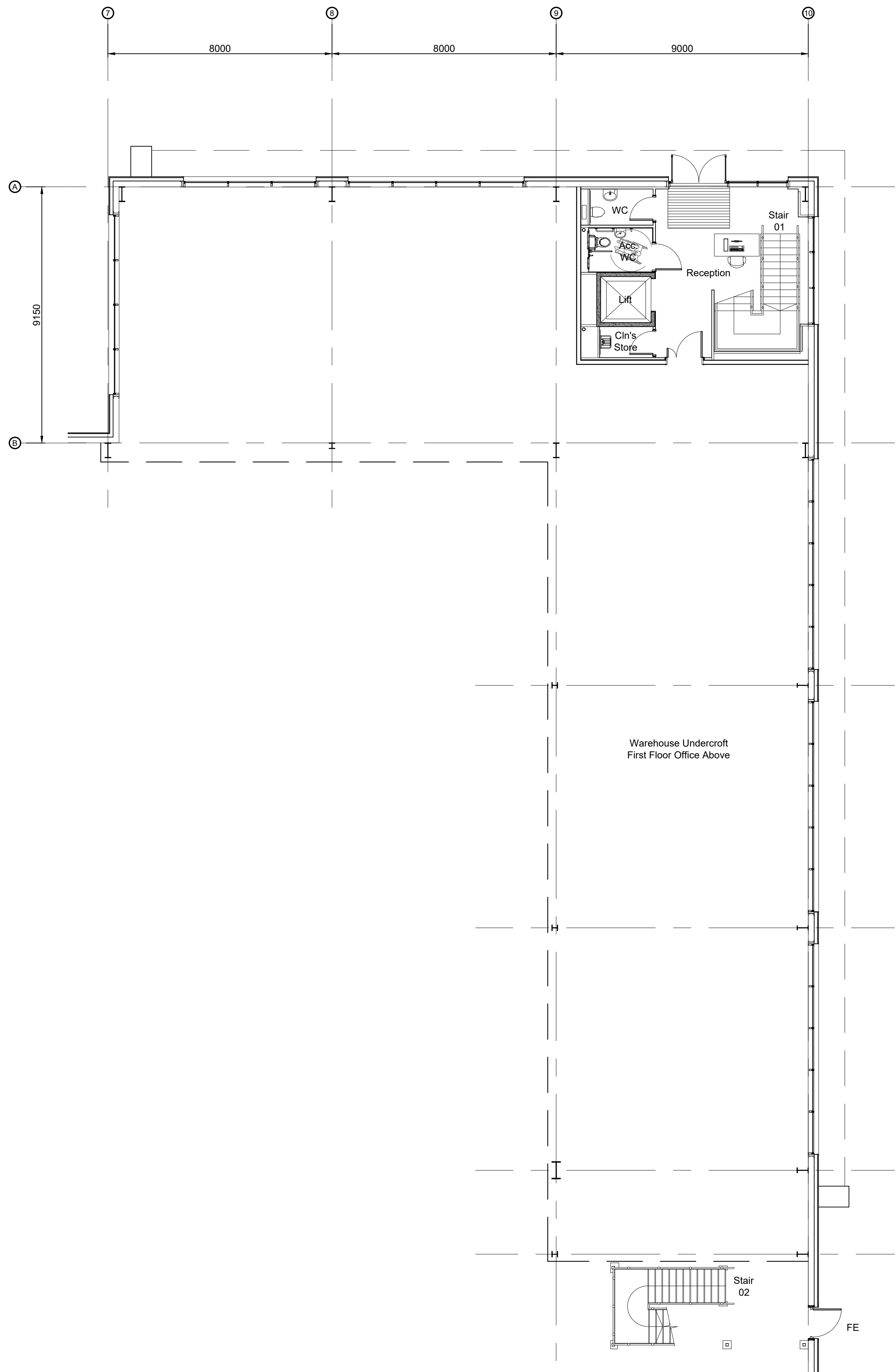
Ground Floor Core & Undercroft Scale 1:100
