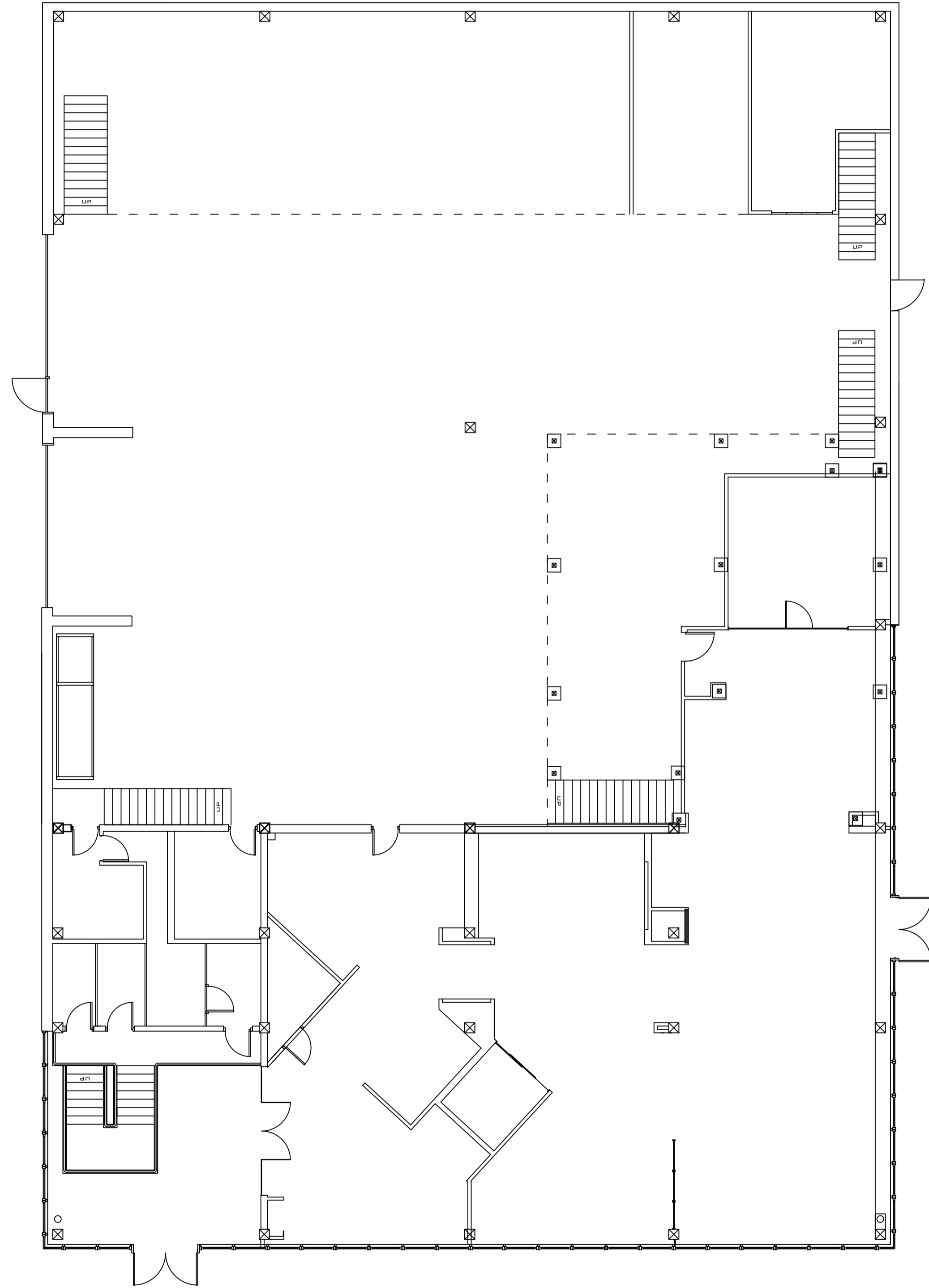
Ground Floor
